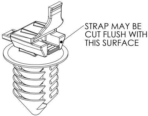
ASSEMBLED VIEW
